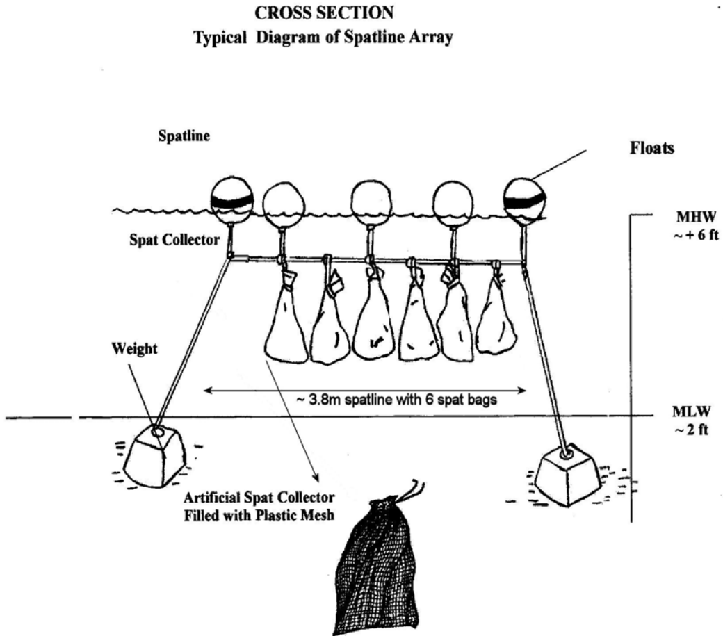
Figure 3. Schematic diagram of spat bag array.
