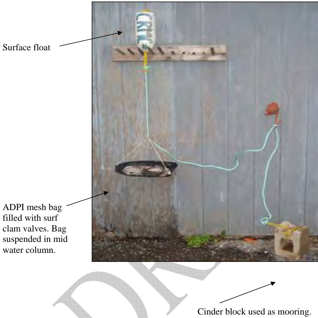
Figure 11. Artificial oyster spat collector used in 2008.
